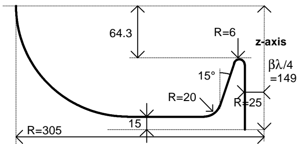
Fig. 1 Optimized 2D cell ( \beta=0.7 )
