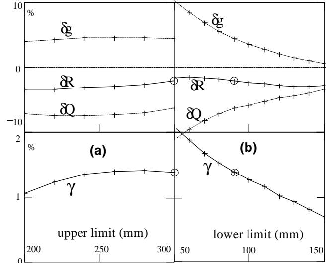
Fig. 5. Influence of slot height. Limits are from the z-axis. The optimized case is circled.
