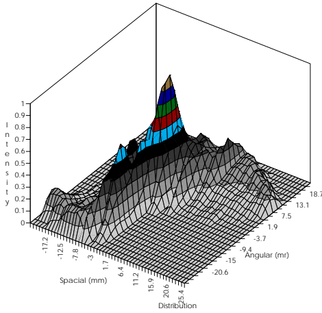
Fig. 3: 20 keV Emittance contour plot.
