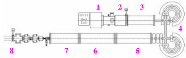
Fig. 1: The BRF PET Linac.
