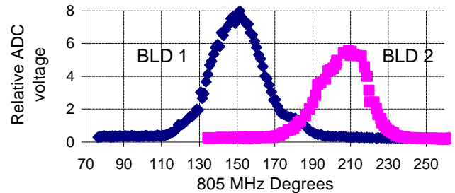
Figure 3, Typical bunch-length measurement.
