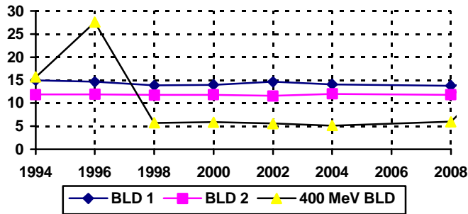
Figure 4, Bunch Length through the macropulse.
