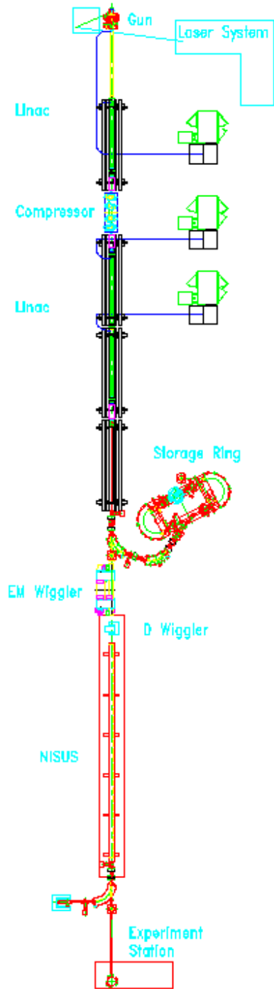
Fig. 1. Layout of SDL linac and experiments.
