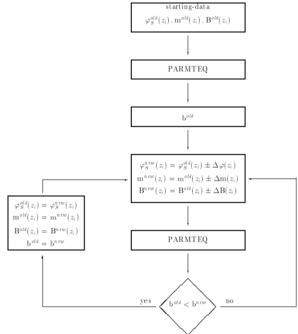
Figure 4: Diagram of the optimizing algorithm.
