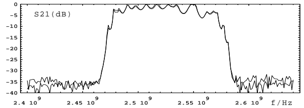
Fig. 1 Transmission through a chain of two TESLA 9-cell copper cavities: Calculated from single cavity measurements and measured directly (two curves)
