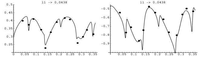
Fig. 7 Typical plot of the input reflection at port B of the complete setup for fixed L_1 against L_2 (comp. Fig. 6)
