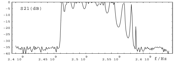
Fig. 2 Transmission through a chain of four TESLA 9-cell copper cavities, calculated from single cavity measurement
