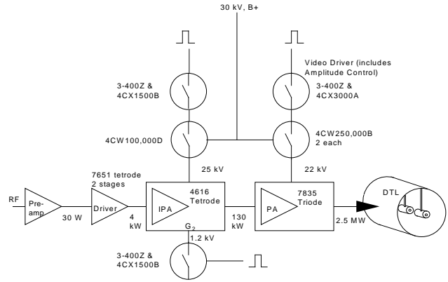
Fig. 1. Original 201 MHz Amplifier System.
