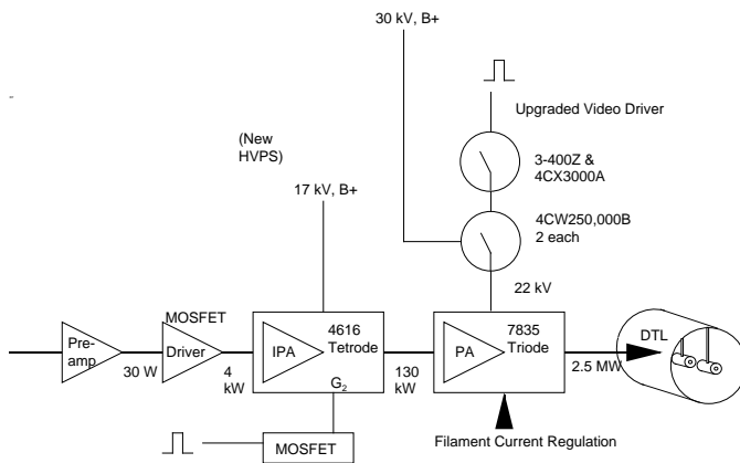
Fig. 2. 'Upgraded' 201 MHz Amplifier System.
