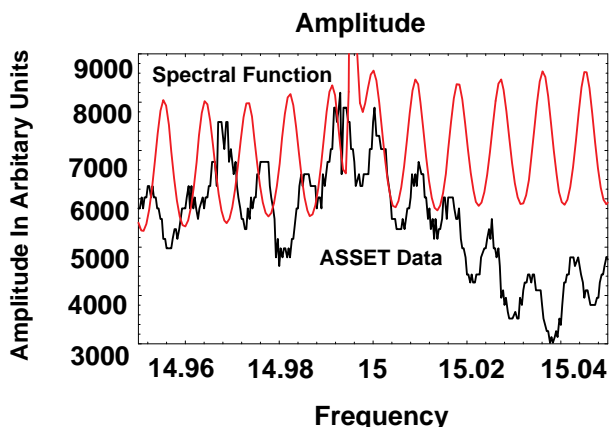
Fig. 5: Fine details of the observed spectrum, compared to theoretical predictions. The mode spacing is slightly smaller than predicted which is compatible with the observation of a somewhat delayed occurrence of the recoherence peak in the ASSET-wakefield measurements [1].
