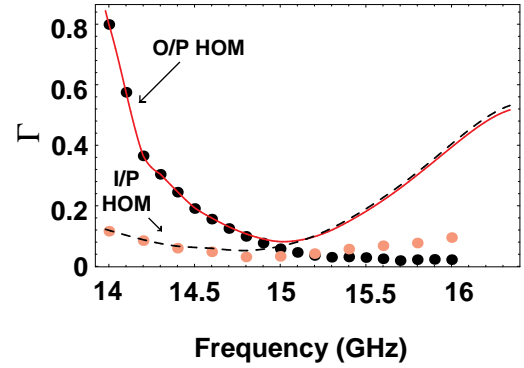
Fig. 3 Reflection coefficient \Gamma_c of the manifold output assemblies looking from the manifold into the mitre bend and the vacuum window, as inferred from bench measurements.
