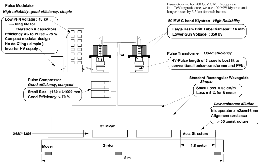
Fig. 2 What makes the C-band system simple and reliable. The key points in the C-band rf-system.
