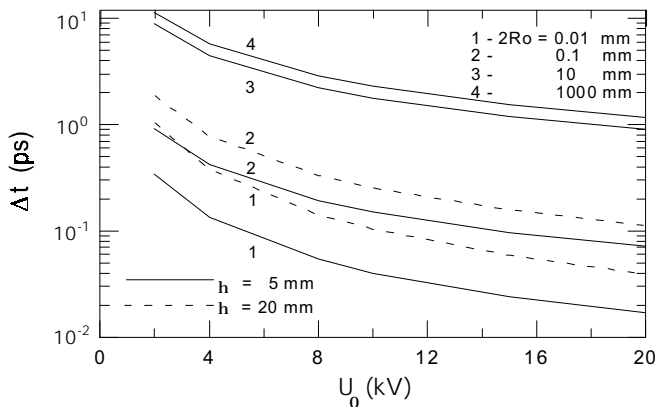
Fig.4. Time spread of secondary electrons in the primary converter vs. the target voltage U_0 for different target radius R_0 and two distances h (see Fig.1.b).
