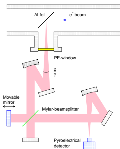
Figure 4: Interferometer setup for bunch length measurement with transition radiation.
