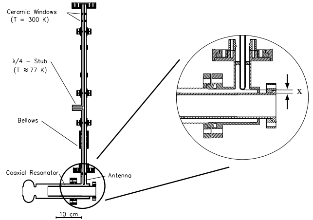
Figure 2: Cut of the tuneable sc input coupler.
