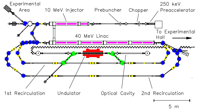
Figure 1: Layout of the S-DALINAC accelerator hall.
