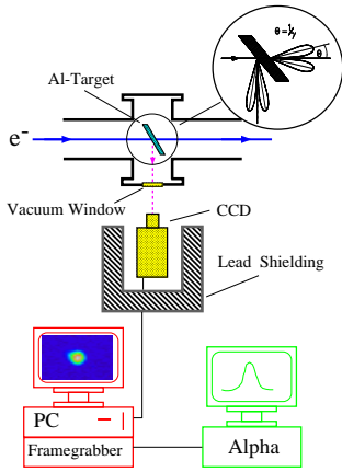
Figure 3: OTR diagnostic station.
