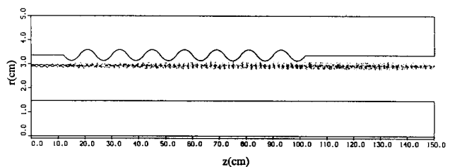
Fig. 4. Particle-in-cell simulation of coaxial geometry showing electron beam with strong axial bunching.
