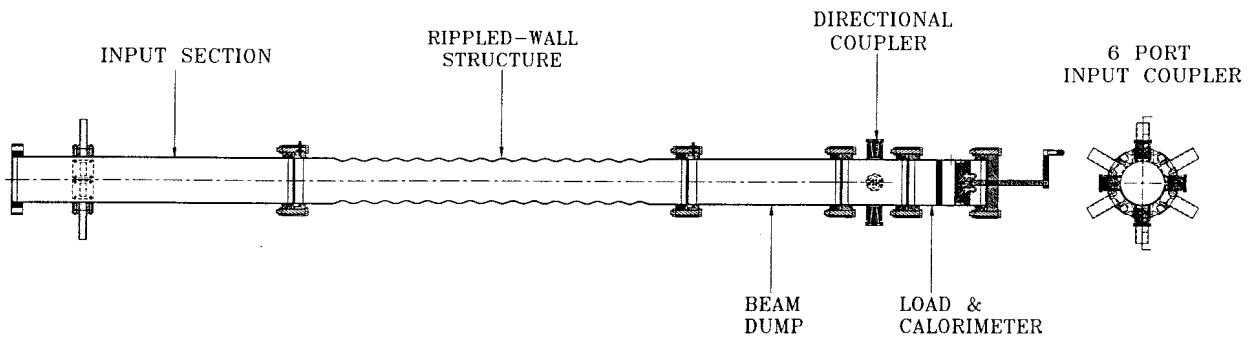
Fig. 5. FEM experimental configuration.
