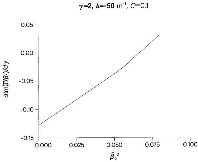
Fig. 1. Sensitivity of phase to beam energy for medium gain and low energy ( \gamma = 2 ) as a function of space charge wavenumber.
