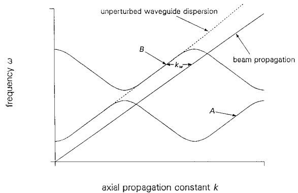
Fig. 3. Generic dispersion relation for a periodic waveguide with small perturbations
