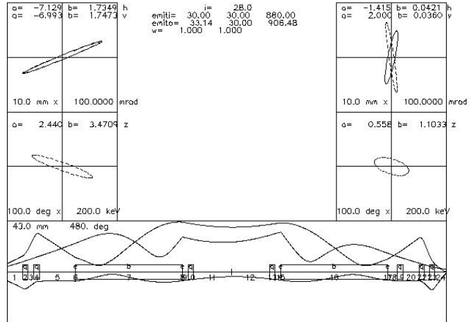
Figure 4 MEBT optics
