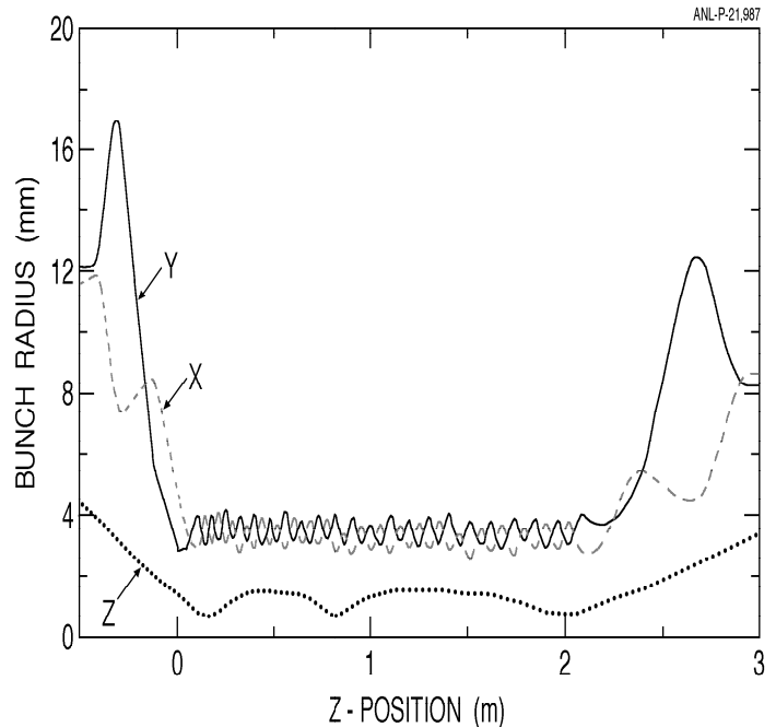
Fig. 2. Transverse and longitudinal beam size through entrance and exit matching electrostatic quad triplets and through the 12 MHz, 2 meter long RFQ structure.
