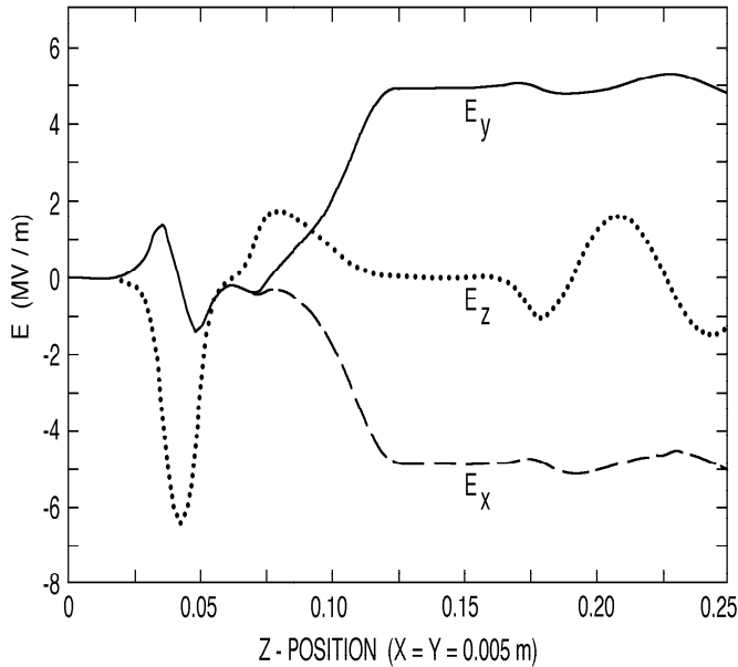
Fig. 1. Electric fields at the entrance of the RFQ, from TOSCA. A drift-tube 20 mm long, centered at z = .06 meters, is tied to the high-voltage vane pair.
