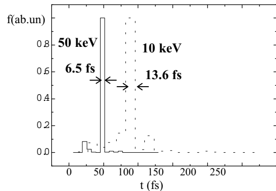
Fig.2. Time distribution of the delta - electrons with energy of 10 and 50keV scattered by the 10 MeV electrons in the carbon fibre of 8 \mu\text{m} diameter.
