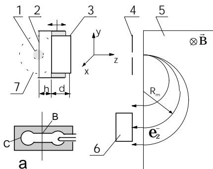
Fig.1. Scheme of bunch phase distribution monitor.
