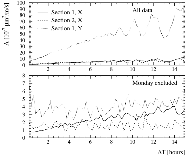
Figure 4: Calculated A constant as a function of the time interval \Delta T in the ATL rule. The three different curves refer to the horizontal (solid) and vertical (dotted) data of section 1 and the horizontal data of section 2 (dashed). The upper results include all data. In the lower case the data between 100 and 120 hours (see Fig. 3) was excluded. The perturbing effect of an FFTB access was such eliminated. The A constant was determined over a distance of approximately twice 15 m.
