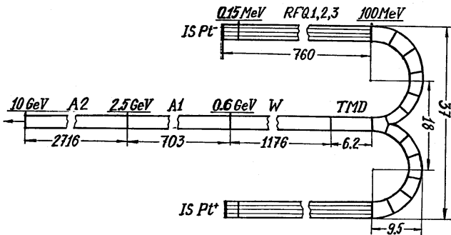
Figure 1: The total scheme of linac: IS -ion sources; RFQ1,2,3 - injector channels; TMD - transverse matching device; W - Wideroe channel; A1 and A2 - Alvarez channels; all lengths are measured in meters.
