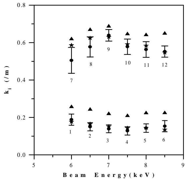
Fig. 5 Amplitude decay rate of fast waves.
