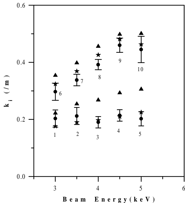
Fig. 4 Amplitude growth rate of slow waves.
