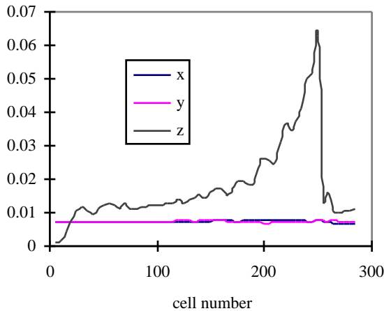
Fig. 2 Transverse and longitudinal emittance evolution for a mono-species beam.
