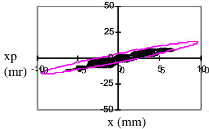
Fig. 4 Measured horizontal emittance , the solid line represents the calculated ellipse.
