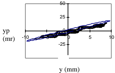
Fig. 5 Measured vertical emittance , the solid line represents the calculated ellipse.
