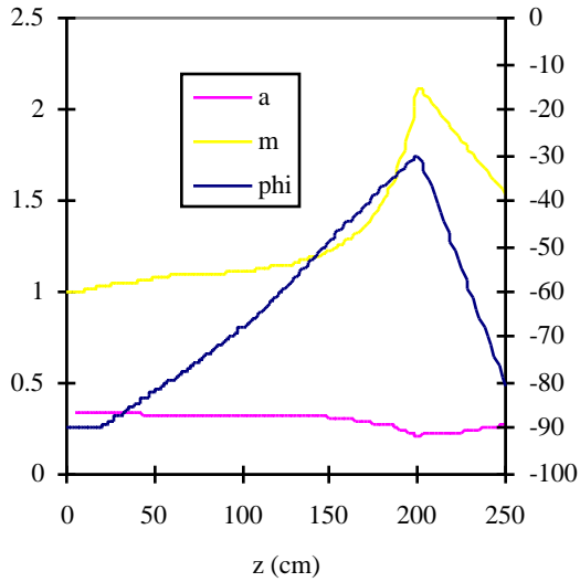
Fig. 1. Variation of RFQ aperture, modulation and phase vs. length. Phase and modulation are tapered down in the last section in order to limit the output energy to 100 keV/u for the first phase of the experiment.
