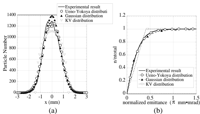
Fig. 3 Comparison of the experimental results with the simulated results; (a) the beam profiles and (b) the relationships between the normalized emittance and the beam fraction in the emittance.
