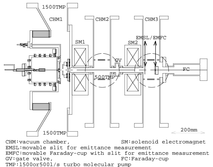
Fig. 1 A schematic drawing of the experimental setup viewing from the upper position.
