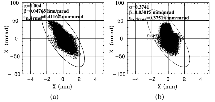
Fig. 2 Particle distributions in the horizontal emittance phase space measured at the entrance of the RFQ; (a) when the vacuum pressure in CHM2 was 3.7 \times 10^{-6} Torr in the typical operation and (b) when it was 3.7 \times 10^{-5} Torr.
