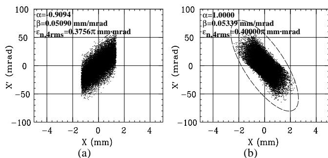
Fig. 4 Particle distributions in the horizontal emittance phase space; (a) the initial distribution generated with UY-dst and (b) the simulated results with an equivalent beam intensity of 1.1 mA at the entrance of the RFQ.
