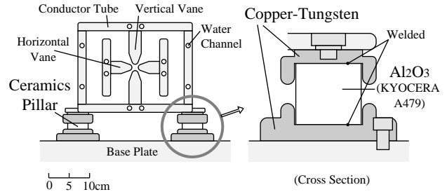
Fig. 3 Schematic drawing of the improved ceramics pillar.
