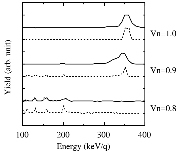
Fig. 6. Measured energy distribution (solid curves) and the PARMTEQ simulation (dashed curves). This measurement was done at the frequency of 17.64 MHz using Ar^{2+} beam. The corresponding output energy is 350 keV/q. The numbers represented by V_n indicate the ratios of the intervane voltage to the standard value of 26.1 kV.
