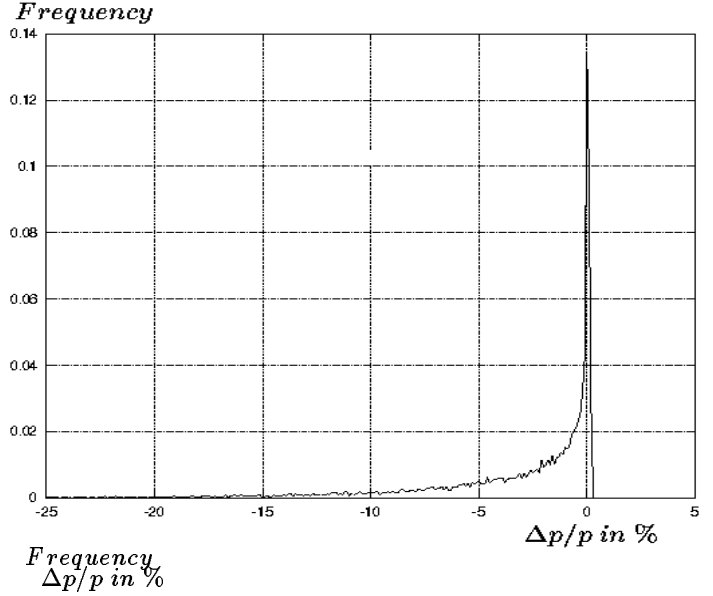
Figure 1: Distribution of energy deviation of the disrupted beam for the TESLA linear collider.
