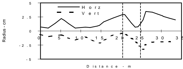
Fig. 2. The design beam envelopes for the new beam line.
