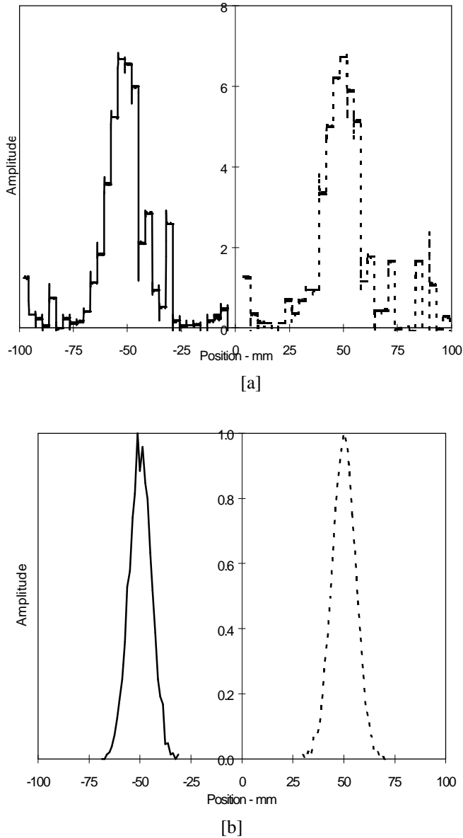
Fig. 4. [a] Observed horizontal profiles at the BIRCMW location in Fig. 1 with octupoles ON (left) and OFF (right). [b] The corresponding profiles predicted by TURTLE.
