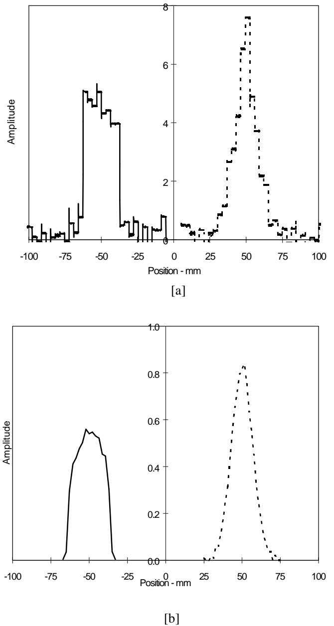
Fig. 5. [a] Observed vertical profiles at the BIRCMW location in Fig. 1, with octupoles ON (left) and OFF (right). The tilt of the vertical ‘flat-top’ was due to vertical mis-steering and could be removed or reversed with the vertical steerers. The downstream quads were set differently than in Fig. 3. [b] The corresponding profiles from TURTLE.
