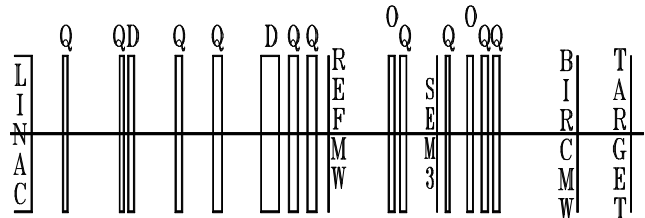
Fig. 1. Schematic layout of the BIRC beam line, showing quadrupoles (Q), octupoles (O), dipole magnets (D) and profile monitors. Total length is 33.5 m, and is to scale horizontally.
