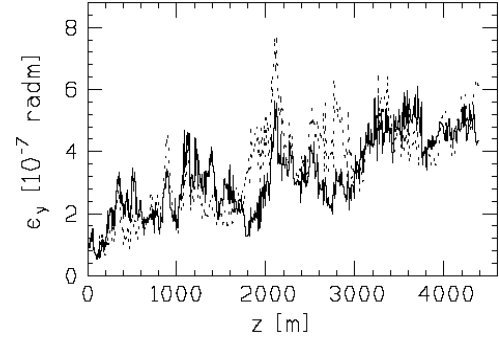
Fig. 1. Evolution of the vertical emittance along the linac with alignment errors of 10 \mu\text{m} rms after: 'one-to few' correction (dotted line) and DF correction (continuous line).
