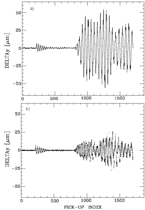
Fig. 5. Effect of a DW correction on: (a) the term describing wake-field effects (b) the terms describing the effects of energy dispersion. Correction is applied over 800 pickups.
