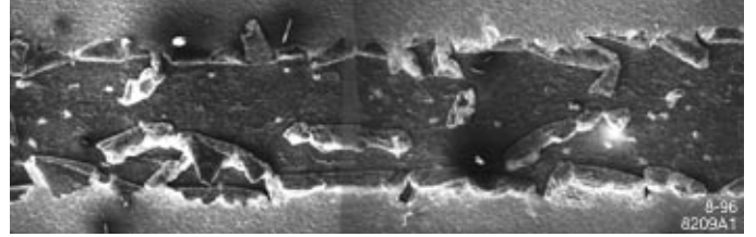
Fig. 1: Damaged collimator surface (stripe width \approx 1 \text{ mm} ). The beam enters at the left, creating gold flakes and spherules.
