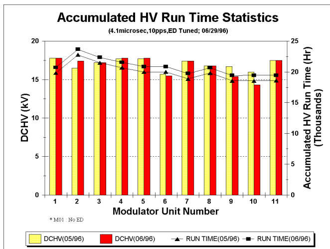
Fig.1: Accumulated run time of klystrons.
