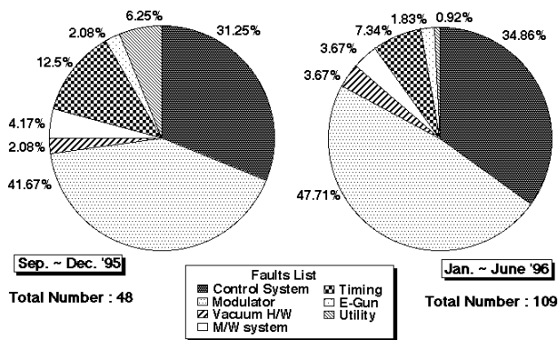
Fig. 2: Relative ratio of the linac operational faults.
