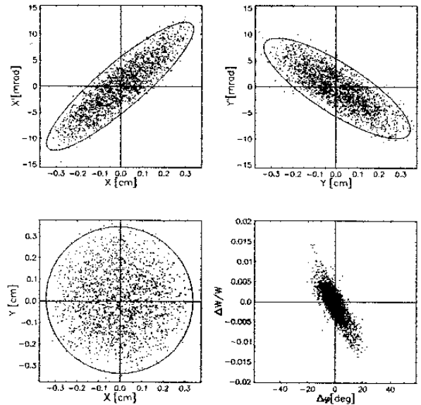
Fig. 4: Output distribution for a 16.5 mA input beam.
