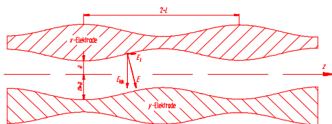
Fig. 1 Scheme of RFQ electrodes.
