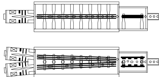
Fig. 5 Scheme of the two beam RFQ.
