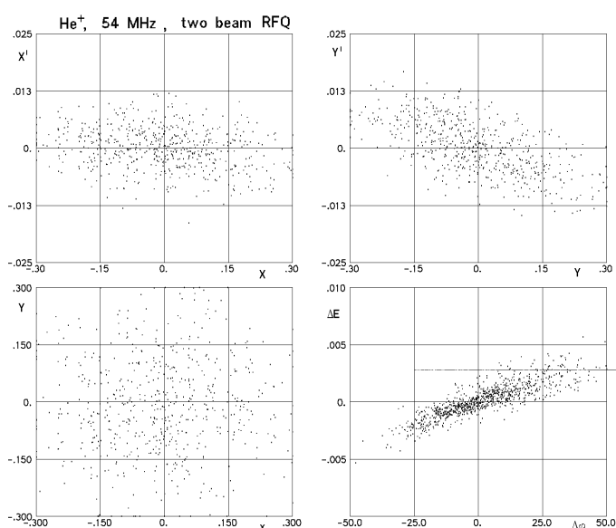
Fig. 6: Output particle distribution for the twin beam RFQ.
