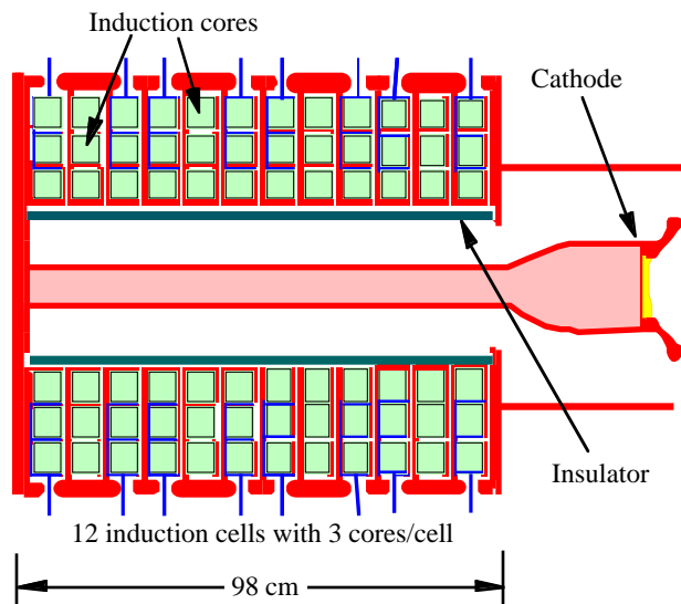
Fig. 4. Schematic of the cathode-half of the RTA gun. This section provides 0.5 MeV of the gun's potential.
