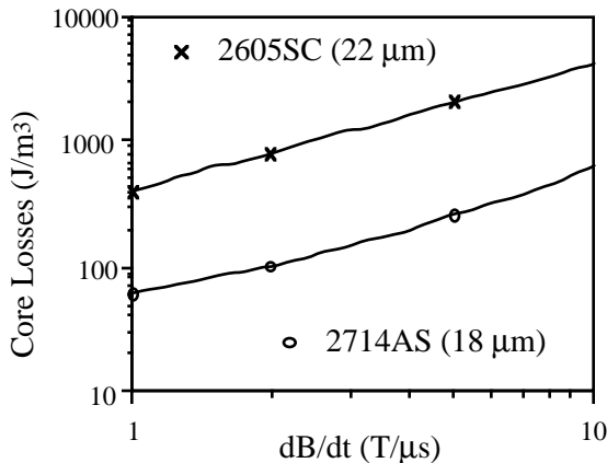
Fig. 2 Core loss for different rates of magnetic flux change.
