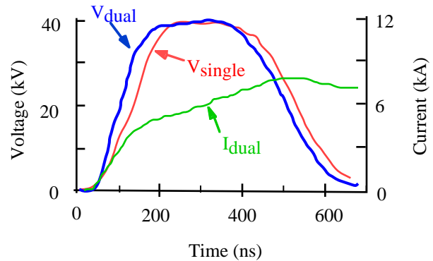
Fig. 3. Cell voltage and drive current for a prototype injector cell.
