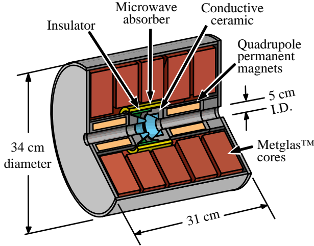
Fig. 1. A proposed RK-TBA induction cell design illustrating longitudinal core segmentation.
