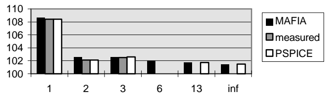
Fig. 3. Frequencies of RFQ models with n cells.
