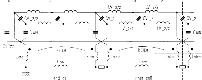
Fig. 5. PSPICE equivalent circuit.
