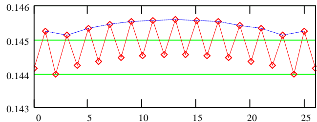
Fig. 4. Voltage variations along 13-cell RFQ.
