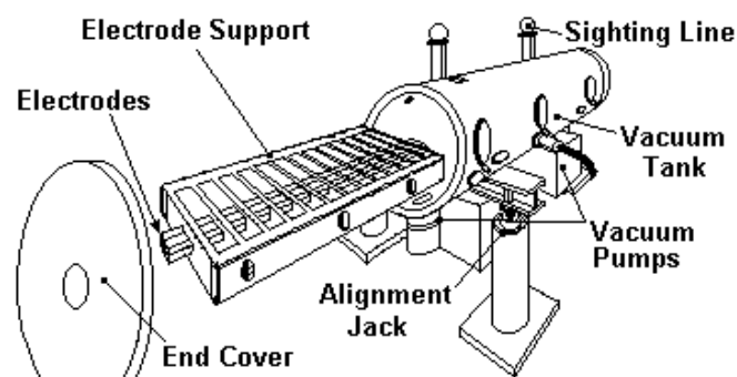
Fig. 1. General assembly of the RFQ.
