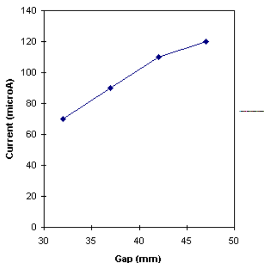
Fig. 3. Pb^{27+} current variation with extraction gap.
