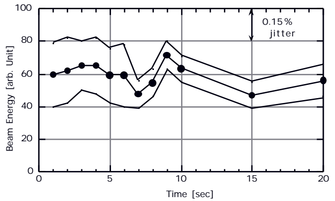
Fig. 6b. Beam energy jitter measured at the end of the PF 2.5-GeV linac. Fast jitter in pulse to pulse disappeared after the beam trigger was resynchronized.
