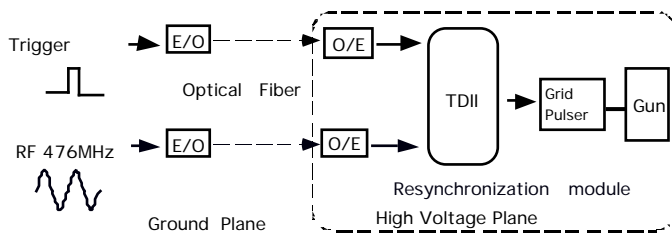
Fig. 2 Schematic diagram of the resynchronization system.
