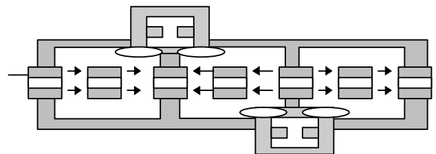
b. Side-coupled structure.
