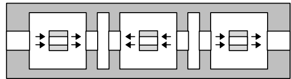
a. On-axis coupled structure
