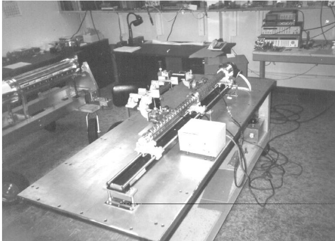
Fig. 3. Two-section linac built for intraoperative therapy. Modified side-coupled structure with Alvarez resonator is incorporated into standard side-coupled structure.
