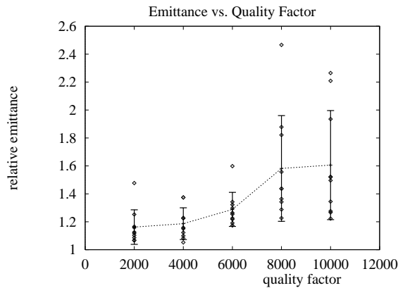
Fig.1: Simulation results for the vertical beam emittance (normalized by the design emittance) at the end of the S-band linac as a function of HOM quality factors.
