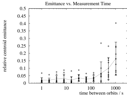
Fig. 2: Emittance growth caused by diffusive ground motion with A=10^{-17} m/s during the process of WF-correction as a function of time between orbit measurements.
