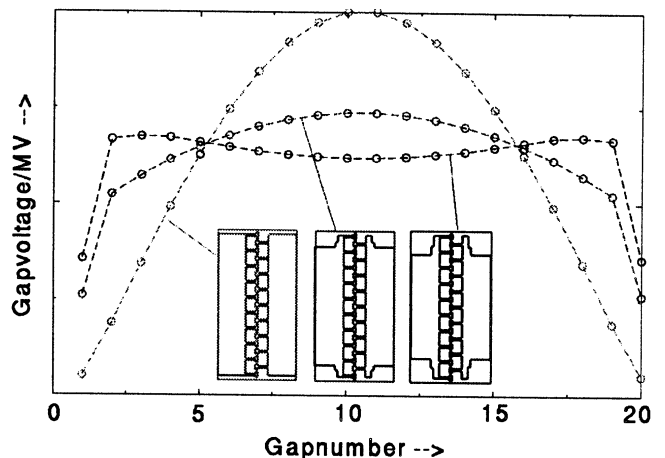
Figure 2: Voltage distribution for different depths of the undercuts in the girders.
