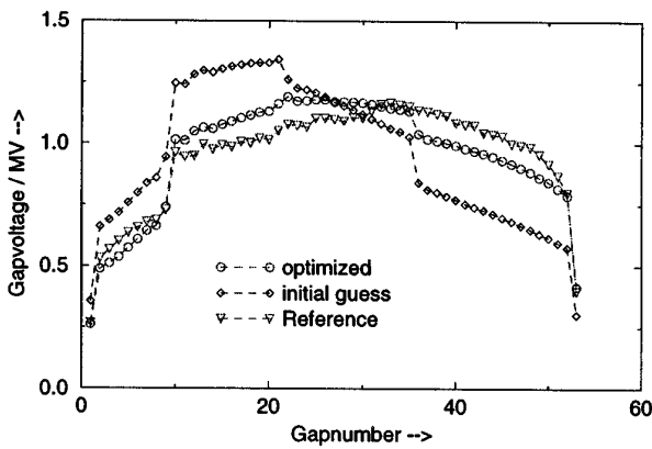
Figure 7: Calculated and reference voltage distributions in cavity IH1.
