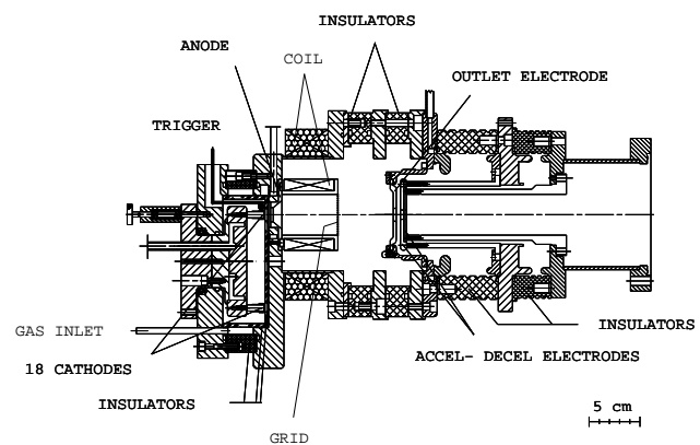
Figure 3: MEVVA ion source.
