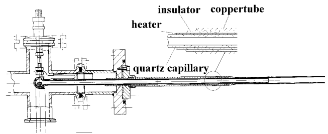
Figure 6: Evaporator for ECR ion source CAPRICE.
