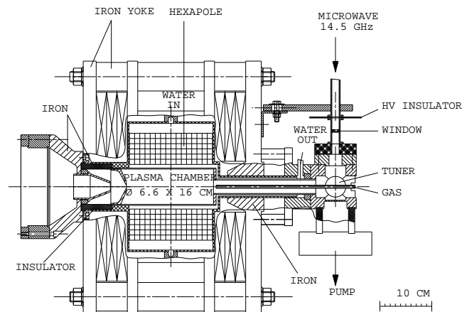
Figure 5: ECR ion source CAPRICE.
