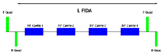
Figure 2: Focusing structure of the linac.
